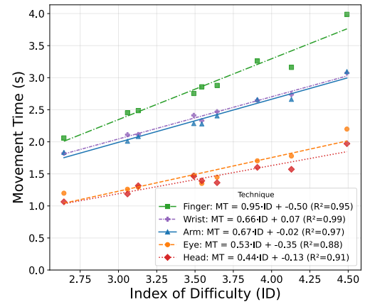
Figure 5: Movement Time vs Index of Difficulty
